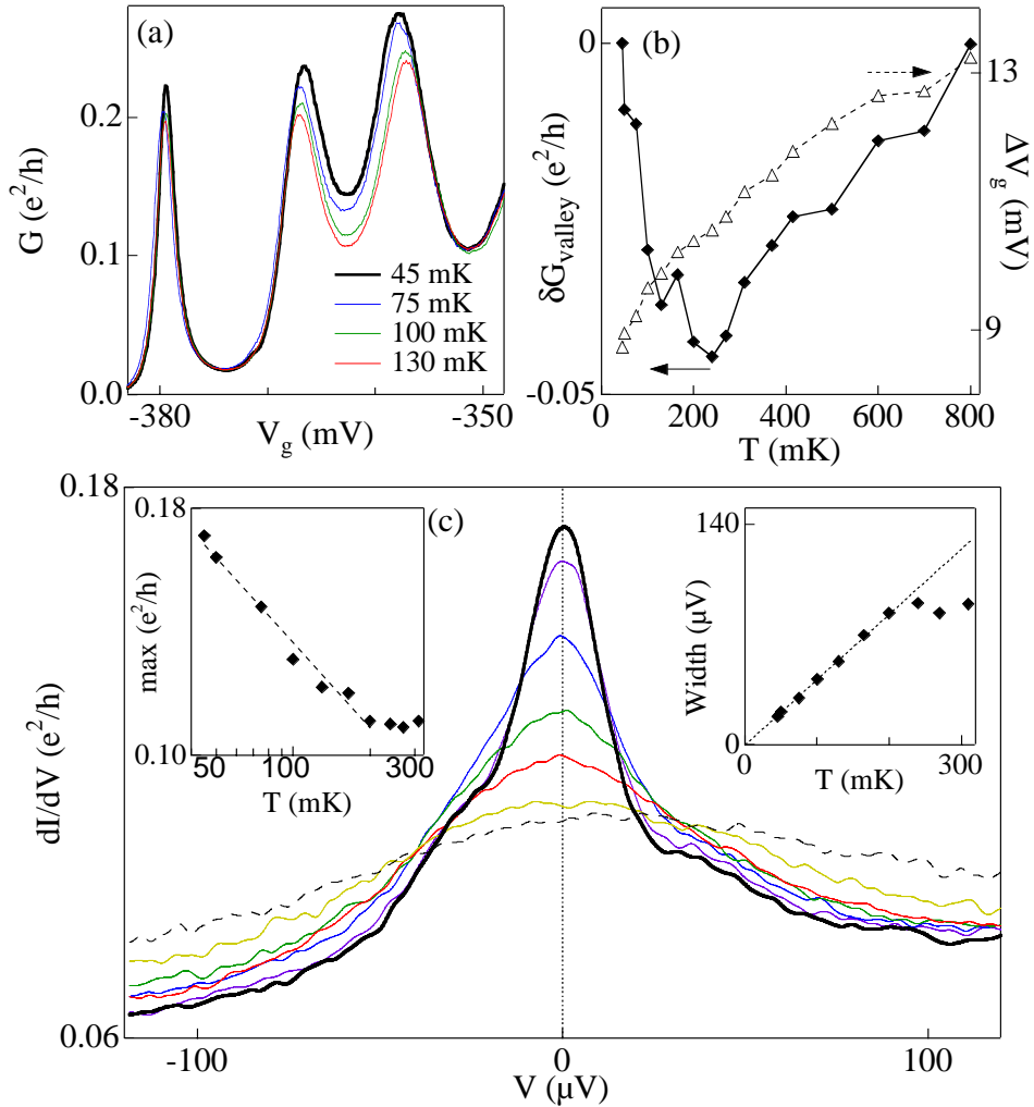
Figure 5-7. (a) Conductance G for B = 0 and V = 5.9 \mu\text{V} at 45 (bold curve), 75, 100 and 130 mK in dot 2. Because dot 2 is smaller, the tunnel barriers increase more rapidly with negative gate voltage, and we observe only three consecutive valleys in the Kondo regime. The middle valley shows pronounced Kondo behavior. (b) Left axis: \delta G_{\text{valley}}(T) ( \blacklozenge ) for the center of the middle, Kondo valley in (a). Right axis: gate voltage spacing \Delta V_g(T) ( \square ) of the peaks bordering the Kondo valley. Increasing T results both in a Kondo minimum in \delta G_{\text{valley}} , and an increasing peak spacing that we ascribe to a renormalization of the energy level \epsilon_0 . (c) Differential conductance dI/dV versus source-drain bias voltage V for T = 45 (bold), 50, 75, 100, 130, 200, and 270 (dashed) mK. The gate voltage is set in the center of the middle valley. The asymmetry in the zero-bias peak is probably because \Gamma_L \neq \Gamma_R . Left inset: The peak maximum is logarithmic in T . Right inset: The peak width (the full-width at three-quarter maximum) is linear in T with a slope of 4.8k_B (dotted line).
