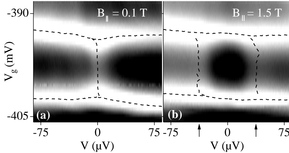
Figure 5-12. Split zero-bias peak independent of gate voltage (a, b) Grayscale plots of dI/dV as a function of V_g and V show the zero-bias peak for B_{\parallel} = 0.1 T split into two shoulder peaks at B_{\parallel} = 1.5 T. White regions mark large dI/dV while black regions indicate low conductance. This valley is the Kondo valley from Fig. 5-7(a). The contour of the CB peaks (horizontal) and the maxima in the dI/dV (vertical) are indicated by dashed lines. The valleys on either side of the Kondo valley do not show a zero-bias or split dI/dV peak. The arrows on the bottom axis of (b) indicate the theoretical splitting, which should be independent of V_g , with a value of \pm 37.5 \mu\text{V} at B_{\parallel} = 1.5 T. The arrows matches the experimental results very well.
