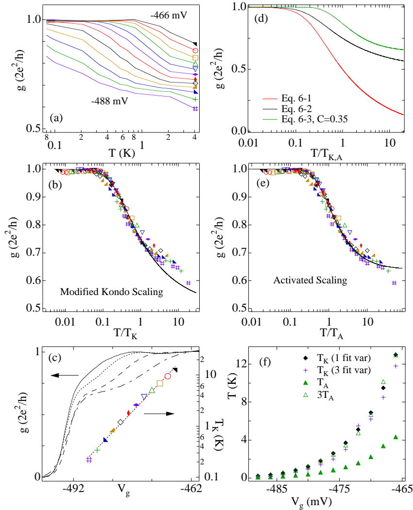
Figure 6-14. g(T) scaled by a T_K and T_A . (a) Raw conductance data g(T) from V_g = -466 mV to -488 mV in 2mV steps. Marker shape and color are kept the same throughout the figure. (b) Linear conductance, g , as a function of scaled temperature T/T_K where T_K is the single fit parameter in Eq. 6.2. When scaled this way, g(T/T_K) collapses to a single curve that agrees well with the modified Kondo form, Eq. 6.2 (solid curve). (c) The values of T_K (markers, right axis) obtained from fits of g(T) to Eq. 6.2. The Kondo temperature, T_K , depends exponentially on V_g ; a line fit to \ln(T_K) vs. V_g (dotted line) gives a slope of 0.18. Several conductance curves (left axis; as in Fig. 6-4a) at temperatures of 80 mK (solid line), 210 mK (dotted), 560 mK (dashed) and 1.6 K (dot-dashed) show the range of gate voltages where scaling was applied. (d) The functional forms of the scaled conductance for Eq. 6.1 with G_0 = 2e^2/h (red), Eq. 6.2 (black), and Eq. 6.3 with C = 0.35 (green) versus the scaled temperature T/T_K or T/T_A . Note the similarity between the modified Kondo form (Eq. 6.2) and the activated form (Eq. 6.3). (e) Linear conductance, g , as a function of scaled temperature T/T_A , where T_A is the activation temperature from the Arrhenius plots, also collapses to a single curve now well-described by the activated form of Eq. 6.3 (solid curve). (f) The values of T_K (diamonds) and T_A (filled triangles) used in the scaling plots above. The values of T_K from the single-parameter fits to Eq. 6.2 (diamonds) are nearly identical to the T_K values (crosses) extracted from Eq. 6.2 when both the prefactor and added constant are also used as fit variables. The values of T_A depend exponentially on V_g and are very close to 1/3 the Kondo temperatures (open triangles show 3T_A ).
