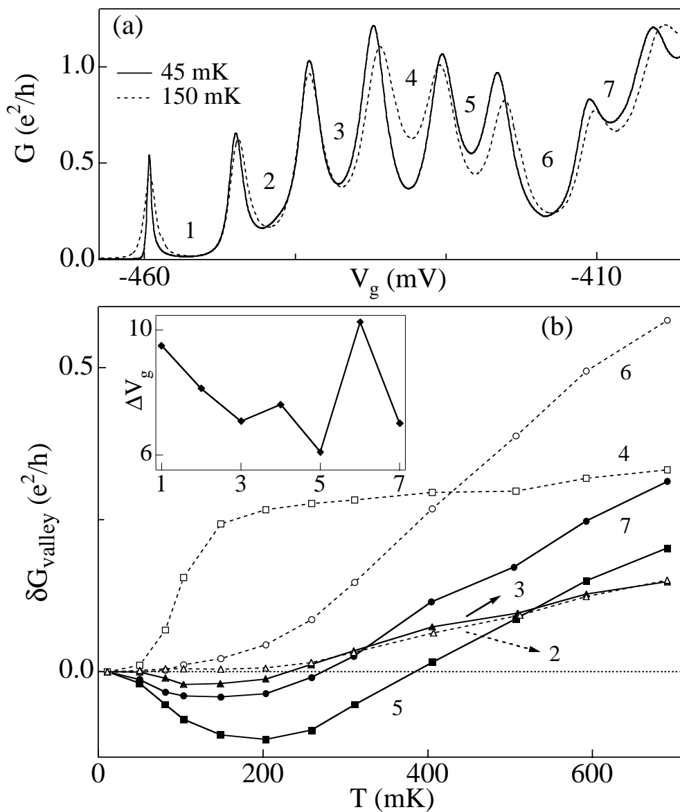
Figure 5-6. Conductance minima in temperature dependence of alternate CB valleys (a) Linear response dc conductance G = I/V versus gate voltage V_g measured in dot 1 at B = 0 for V = 7.9 \mu\text{V} at 45 mK (solid) and 150 mK (dashed). The parity of the valley numbering is indicated by an odd or even number N . From left to right, the CB peaks become broader (i.e. \Gamma is increasing) because the tunnel barrier induced by gates 1 and 2 decreases when increasing the voltage on gate 1. Increasing T from 45 to 150 mK increases the conductance of the even numbered valleys but decreases the conductance of valleys 3, 5 and 7. The detailed temperature dependence is shown in (b) where we plot the change in valley conductance \delta G_{\text{valley}}(T) = G_{\text{valley}}(T) - G_{\text{valley}}(T_{\text{base}}) with T_{\text{base}} \approx 45 mK. The inset to (b) shows the spacings \Delta V_g between adjacent peaks. We observe a larger (smaller) peak spacing for even (odd) N .
