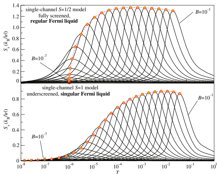
Figure A.1. Spin Seebeck coefficient for the single-channel Kondo model with S = 1/2 (top) and S = 1 (bottom). The magnetic field ranges from B = 10^{-7} to 10^{-1} in steps of factor 10^{1/4} .
