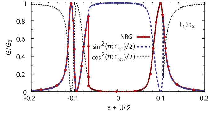
Fig. 6. The conductance G calculated directly from the spectral function by NRG method as a function of gate-voltage \epsilon + U/2 for U/D = 0.2 , r/D = 0.012 , t_1/D = 0.01 , and t_2/D = 0.005 . It is compared with the conductance deduced from the Friedel–Luttinger sum rule, Eq. (4), to indicate the phases of the system.
