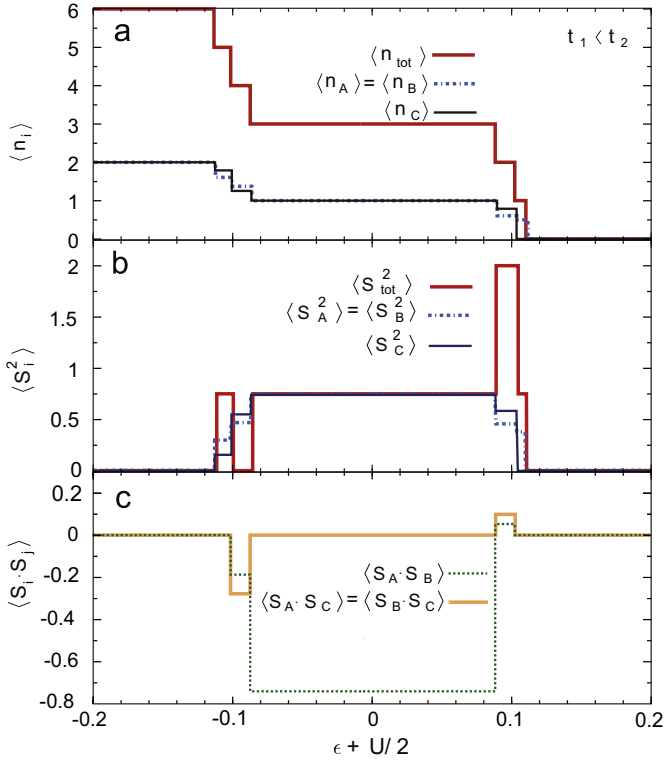
Fig. 3. The quantities: \langle n_{tot} \rangle , \langle n_i \rangle (a), \langle S_{tot}^2 \rangle , \langle S_i^2 \rangle (b) and \langle \mathbf{S}_i \cdot \mathbf{S}_j \rangle (c) with respect to \epsilon + U/2 for the case t_1/D = 0.005 < t_2/D = 0.01 for the isolated TQD. In the middle of the plot, where \langle n_{tot} \rangle = 3 , the ground state is the doublet |D_S^{z=0}\rangle with perfect entanglement between the spins A and B, \langle \mathbf{S}_A \cdot \mathbf{S}_B \rangle = -3/4 , whereas the spin C is decoupled, \langle \mathbf{S}_A \cdot \mathbf{S}_C \rangle = \langle \mathbf{S}_B \cdot \mathbf{S}_C \rangle = 0 . Notice that for \langle n_{tot} \rangle = 1 the dark state occurs for which the dot C is empty and the electron is distributed between the dots A and B.
