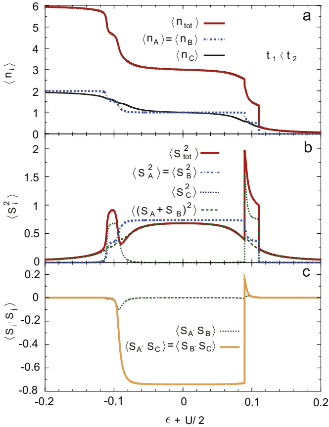
Fig. 5. The quantities \langle n_{tot} \rangle , \langle n_i \rangle (a), \langle \mathbf{S}_{tot}^2 \rangle , \langle \mathbf{S}_i^2 \rangle (b) and \langle \mathbf{S}_i \cdot \mathbf{S}_j \rangle (c) derived by the NRG method for the case t_1/D = 0.005 < t_2/D = 0.01 . The other parameters are the same as in Fig. 4. Note the sharp transition from 1 to 2 electrons at \epsilon + U/2 \approx 0.105 due to the dark state formation, and the transition from 2 to 3 electrons at \epsilon + U/2 \approx 0.09 . Between these two points the spin of the pair of dots A–B is enhanced, \langle \mathbf{S}_{tot}^2 \rangle \rightarrow 2 .
