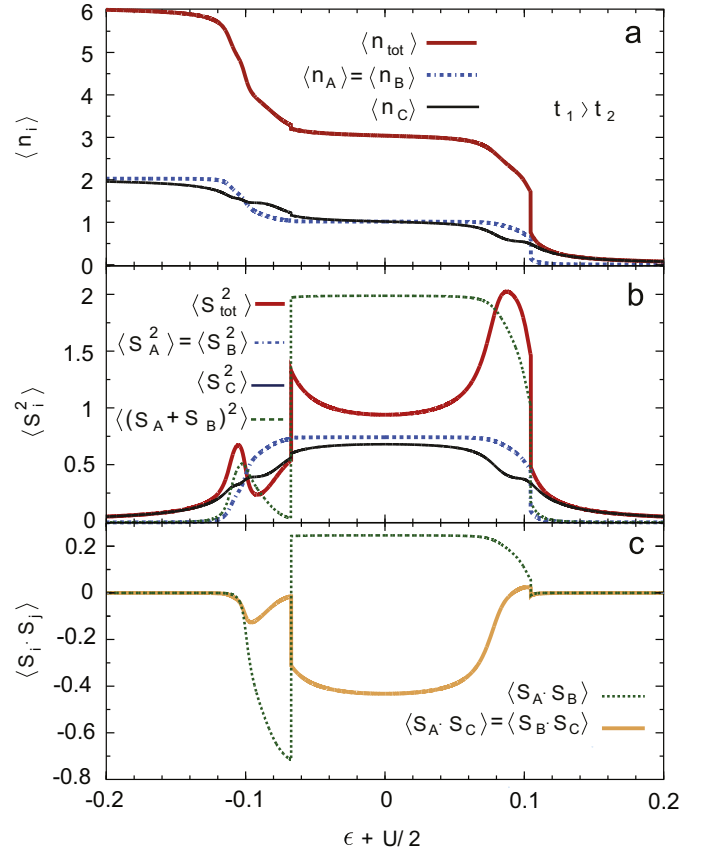
Fig. 4. The quantities \langle n_{tot} \rangle , \langle n_i \rangle (a), \langle S_{tot}^2 \rangle , \langle S_i^2 \rangle (b) and \langle \mathbf{S}_i \cdot \mathbf{S}_j \rangle (c) derived with respect to \epsilon + U/2 by the NRG method for the case t_1/D = 0.01 > t_2/D = 0.005 . The coupling of TQD with the electrodes is taken as r/D = 0.012 and U/D = 0.2 . Compared to the low U/D results here transitions between different regimes are gradual except at particular points \epsilon + U/2 \approx 0.103 and -0.07 , the transition from 2 to 3 electron state where the triplet state is formed and the crossover from 3 to 4 electrons, respectively. The formation of local moments is evident from panel (b) and spin–spin arrangements from panel (c).
