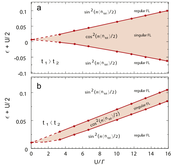
Fig. 8. Phase diagram obtained by means of the NRG code for the TQD molecule coupled with the electrodes, \Gamma/D = 0.012 , where solid curves separate regular Fermi liquid and singular Fermi liquid regions. (a) presents the case with t_1/D = 0.01 , t_2/D = 0.005 , while (b) the case: t_1/D = 0.005 and t_2/D = 0.01 .
