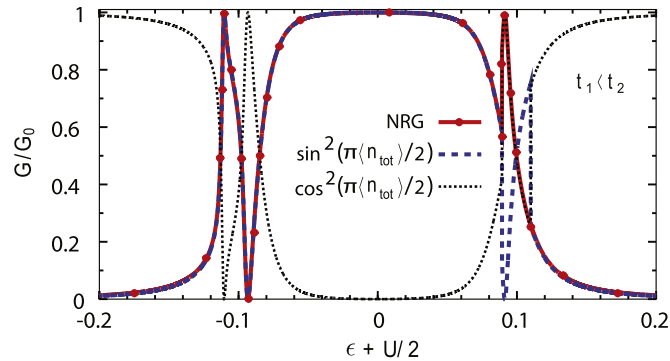
Fig. 7. The conductance G calculated directly from the spectral function by NRG method as a function of gate-voltage \epsilon + U/2 for U/D = 0.2 , \Gamma/D = 0.012 , t_1/D = 0.005 , and t_2/D = 0.01 . It is compared with the conductance deduced from the Friedel–Luttinger sum rule, Eq. (4), to indicate the phases of the system.
