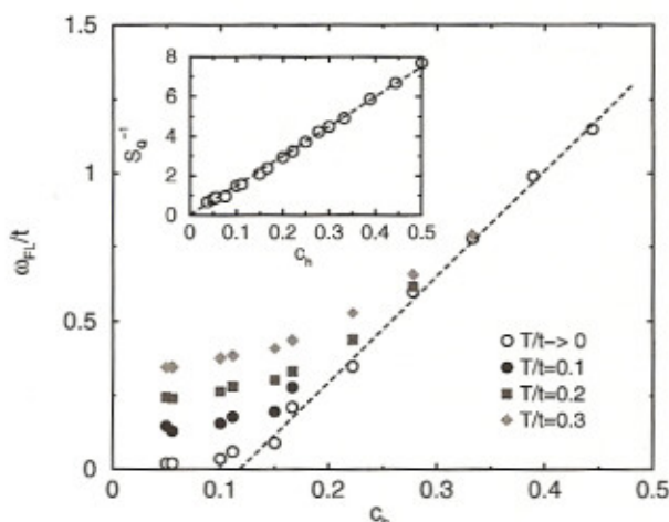
FIGURE 1. FL scale \omega_{FL}/t vs. c_h , obtained for the t - J model using the FTLM for T > 0 and their T \rightarrow 0 extrapolated values. The inset shows T = 0 results for 1/S_Q vs. c_h . Dashed lines are guide to the eye only.
