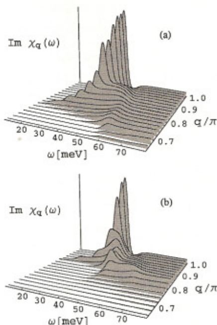
FIGURE 3. \chi''_q(\omega) at intermediate doping c_h = 0.15 for momenta: a) along the x direction \mathbf{q} = q(1,0) , and b) along the zone diagonal \mathbf{q} = q(1,1) .
