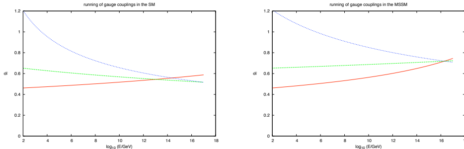
Figure 1: The running of the gauge couplings in SM (left) and low energy MSSM (right).
