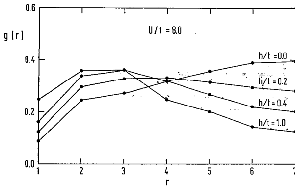
FIG. 3. Hole density-density correlations g(r) vs r for two holes in the Hubbard model with U/t=8 and for different values h/t . Results are for the chain length N=14 .
