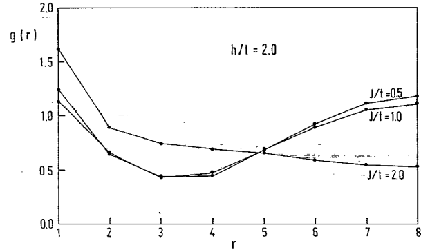
FIG. 2. Same as in Fig. 1, but for N_h=4 and at fixed staggered field h/t=2 .
