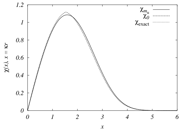
FIG. 1: Comparison of the Langer WKB solution \chi_0 (dashed curve), the exact solution \chi_{\text{exact}} (dotted curve) and the first QLM iterate \chi_{m_u} (solid curve) for the ground state of the anharmonic oscillator V(r) = \frac{1}{2}r^5 . The last two are indistinguishable on the plot. Here x = \kappa r , \kappa^2 = 2mE/\hbar^2 .
