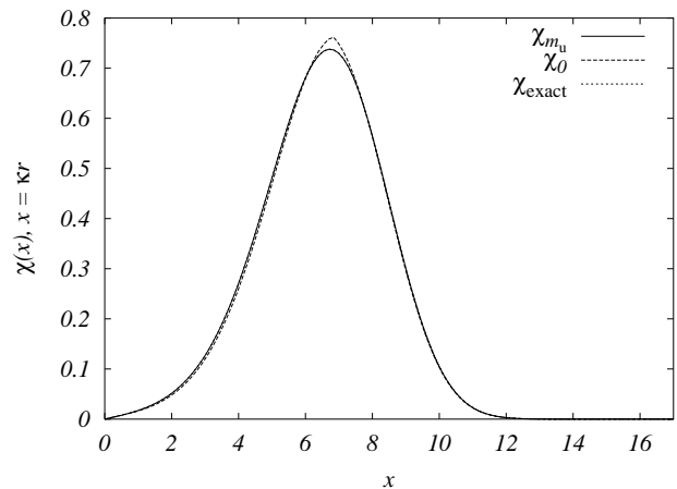
FIG. 16: As in Fig. 1, but for the ground state of the two-power potential V = \frac{1}{2}g^2(r^2 - a^2)^2 , g^2 = 1/4a^2 , a = 4 , or for the first (antisymmetric) excited state of the corresponding double-well potential in one dimension.
