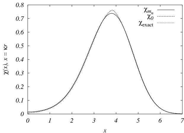
FIG. 14: As in Fig. 1, but for the ground (symmetric) state of the double-well potential V = \frac{1}{2}g^2(r^2 - a^2)^2 , g^2 = 1/4a^2 , a = 4 in one dimension.
