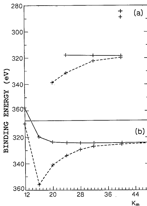
FIG. 1. Binding-energy eigenvalues \epsilon (dashed lines) and their expectation values \langle h \rangle (solid lines), in eV as a function of the maximum global momentum K_m . (a) \mu dt ground state; the two points near the top correspond to the excited state, the plotted values being \epsilon + 250 eV (lower point), and \langle h \rangle + 250 eV (upper point). (b) \mu dd ground state, from Ref. 6, for comparison of the convergence patterns.
