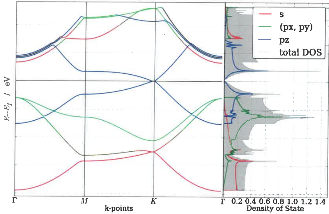
Bands diagram of graphene
