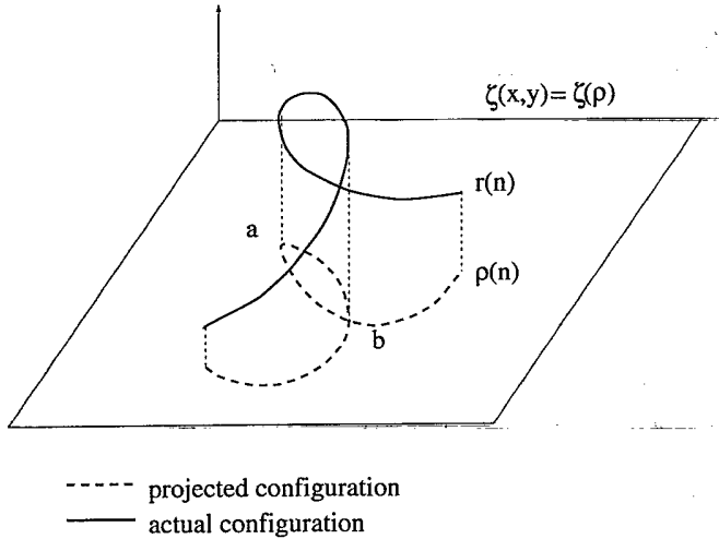
FIG. 1. A 3D polymer configuration projected onto a (planar) surface \zeta(x, y) . Though 3D configuration ( r(n) ) could be of low energy, its projection onto a surface ( \rho(n) ) causes it to become energetically very costly. The region marked (a) is not favored by the elastic energy and the region marked (b) is not favored by the intersegment repulsions. Exclusion of the (a)-type configurations is the origin of the Casimir nematic attraction addressed here.
