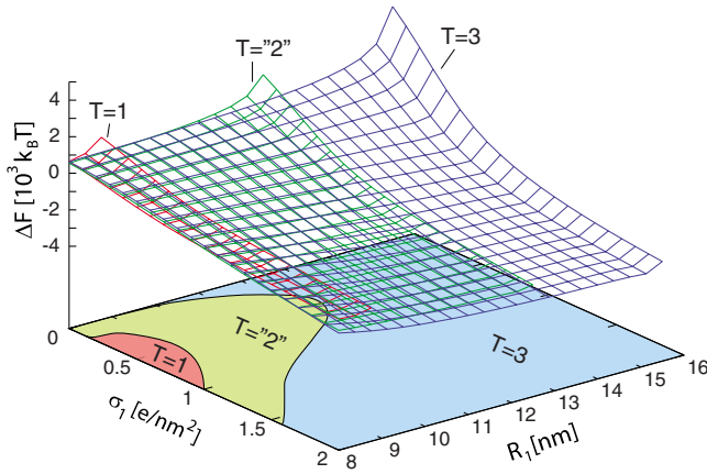
FIG. 4. (Color online) Assembly free energies calculated as functions of the core radius R_1 , its charge \sigma_1 , and for three different capsid radii R_2 (and N_p ), as quantified by three different T numbers. The parameters of this calculation are a=0.5 nm, p=1 , v=0.5 nm 3 , c_0=100 mM, and N_l=18 .
