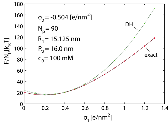
FIG. 2. (Color online) Comparison of the numerically exact results with the analytical DH expression (A9) for the free energy of the capsid with the charged core (complex free energy). The free energy per protein subunit is plotted as a function of the core surface charge density \sigma_1 . The parameters of the calculation are denoted in the figure.
