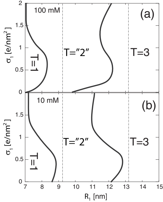
FIG. 10. Regions in the R_1 - \sigma_1 space in which a particular T -number structure has the lowest free energy, as denoted. (a) and (b) show the results for monovalent concentrations of c_0 = 100 mM and c_0 = 10 mM, respectively. The two vertical dashed-dotted lines denote the radii of T=1 and “2” structures ( R_2 ).
