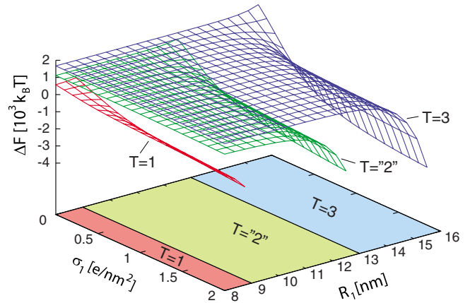
FIG. 3. (Color online) Numerically exact results for the assembly free energy [Eq. (21)] assuming tail-less protein subunits ( c_0=100 mM). The free energies were plotted for capsids with three different T numbers as functions of the core surface charge density \sigma_1 and radius R_1 . The number of subunits and corresponding capsid radii are N_p=30 ( T=1 ), 60 ( T=2 ), and 90 ( T=3 ), and R_2=9.24 ( T=1 ), 13.06 ( T=2 ), and 16 ( T=3 ) nm.
