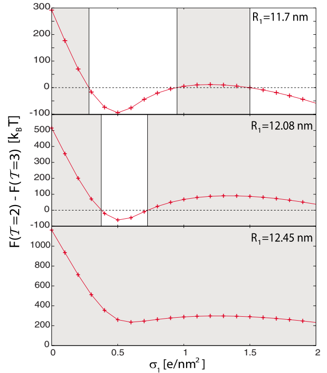
FIG. 9. (Color online) The difference of complex free energy of T=2 and T=3 structures for three different core radii in the transition region as a function of core surface charge density. The parameters of the polyelectrolyte are the same as before and the calculations were performed for the constrained polyelectrolyte model (maximal extensibility limit obeyed). Gray regions denote the surface charge densities \sigma_1 where the T=3 structure has lower free energy.
