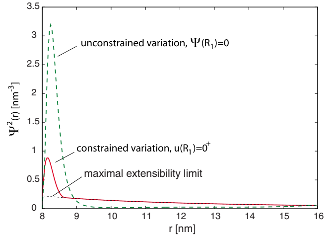
FIG. 7. (Color online) Comparison of the unconstrained monomer density (thick dashed line) and constrained monomer density (full line) approaches. The parameters of the calculation are \sigma_1=1.5e/\text{nm}^2 , c_0=100 mM, R_1=8 nm, R_2=16 nm, N_p=90 , and N_t=18 . The maximal extensibility limit [Eq. (10)] is denoted by a thin dashed line.
