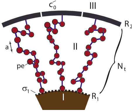
FIG. 1. (Color online) Illustration of the portion of the spherical complex of proteins with flexible tails and a charged core. The parameters discussed in the text are indicated. The configuration of the tails corresponds to the case when the core is poorly charged. For the sake of a clear insight, the illustration shows a discretized model of the polyelectrolyte, although our theory is based on the continuous polyelectrolyte representation (see text).
