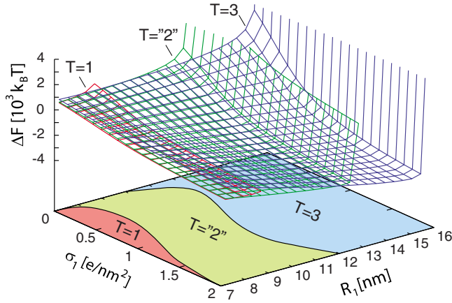
FIG. 5. (Color online) Assembly free energies as functions of the core radius R_1 , its charge \sigma_1 , and for three different capsid radii R_2 (and N_p ), as quantified by three different T numbers. The maximal extensibility ansatz was used to obtain these results. The parameters of this calculation are a=0.5 nm, p=1 , v=0.5 nm 3 , c_0=100 mM, and N_t=18 .
