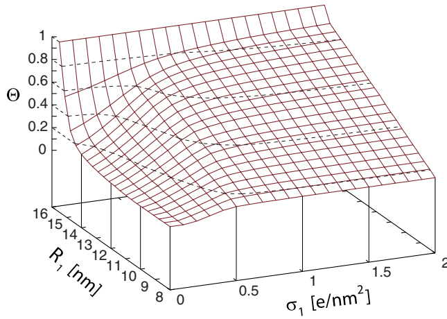
FIG. 8. (Color online) Coverage of the core defined by Eq. (24) as a function of \sigma_1 and R_1 for a complex with T=3 capsids ( R_2 = 16 nm). The calculation was performed with the maximal extensibility constraint on the polyelectrolyte amplitude.
