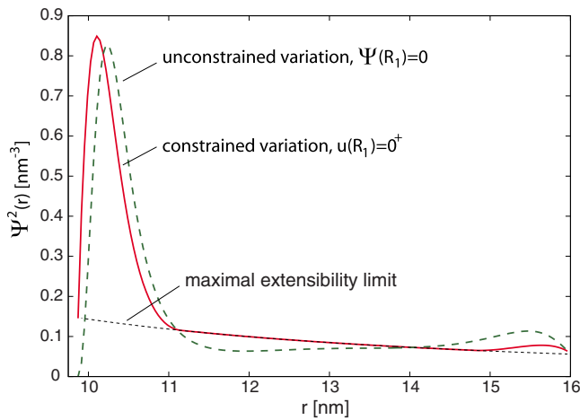
FIG. 6. (Color online) Comparison of the unconstrained monomer density (thick dashed line) and constrained monomer density (full line) approaches. The parameters of the calculation are \sigma_1=0.5e/\text{nm}^2 , c_0=100 mM, R_1=9.875 nm, R_2=16 nm, N_p=90 , and N_t=18 . The maximal extensibility limit [Eq. (10)] is denoted by a thin dashed line.
